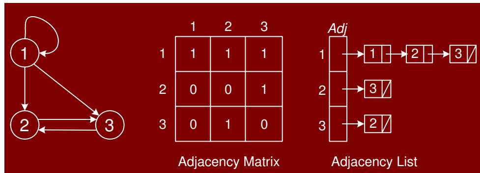
Figure 8.6: Graph Representations
