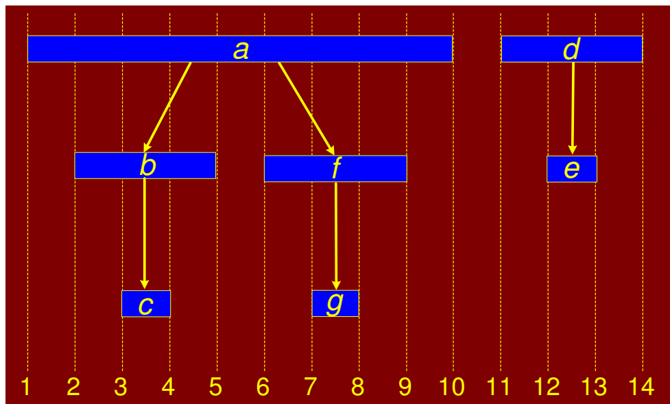
Figure 8.26: Parenthesis lemma
