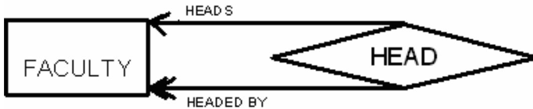
Fig-5: Roles in a unary relationship
